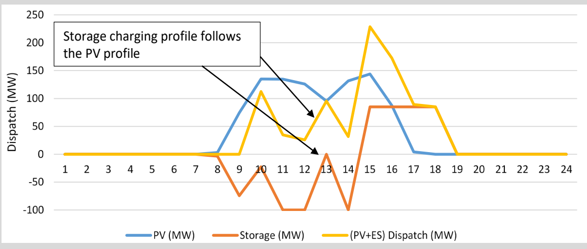
Restricted Storage Charging from Grid (Jan 11)
